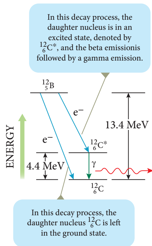
Figure 9.25 Gamma emission
