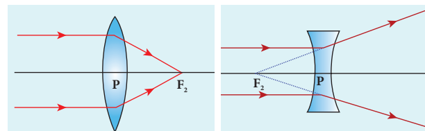
Figure 6.33 Secondary focus
