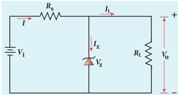
Figure 10.21 Circuit to study voltage regulation by Zener diode
