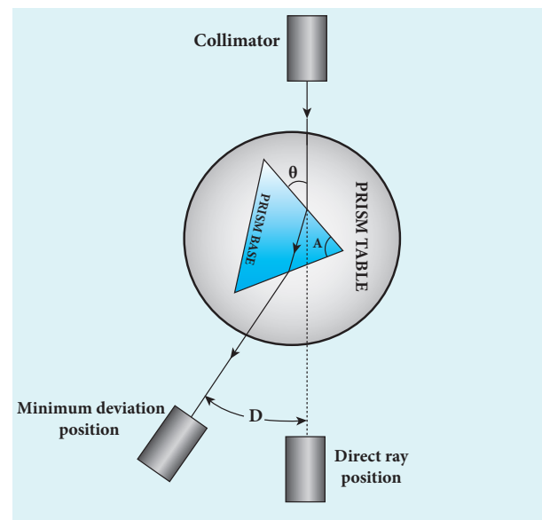
Figure 7.45 Angle of minimum deviation
