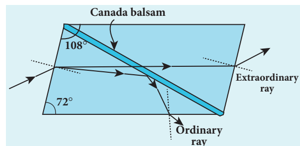
Figure 7.34 Nicol Prism
