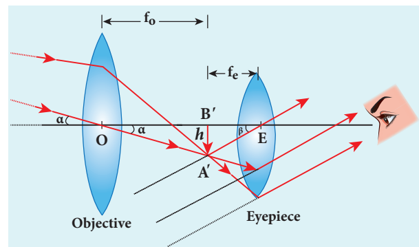
Figure 7.40 Astronomical telescope
