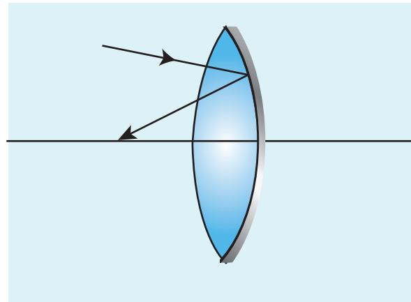
Figure 6.38 Silvered lens
