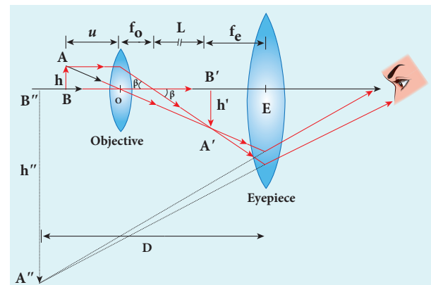
Figure 7.39 Compound microscope
