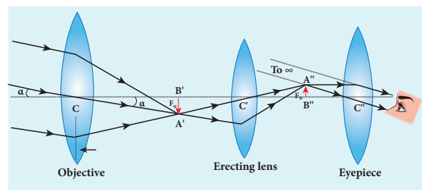
Figure 7.41 Terrestrial telescope
