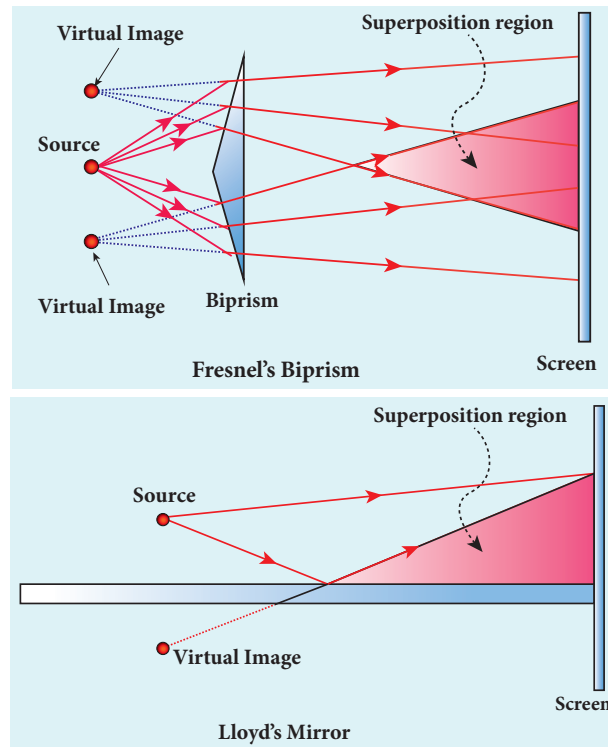
Figure 7.10 Source and images as coherent sources
