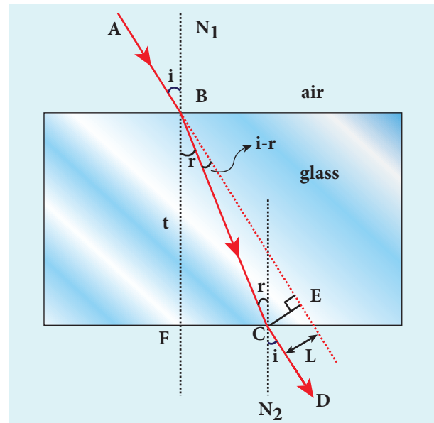
Figure 6.30 Refraction in glass slab
