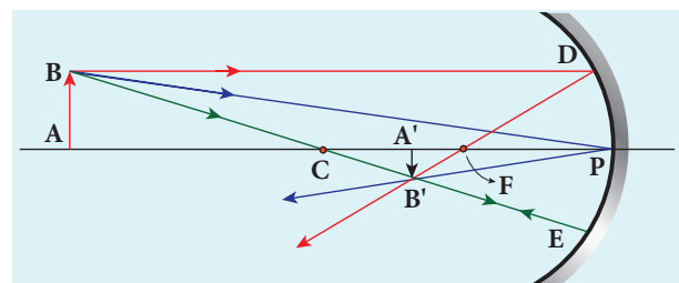
Figure 6.12 Mirror equation
