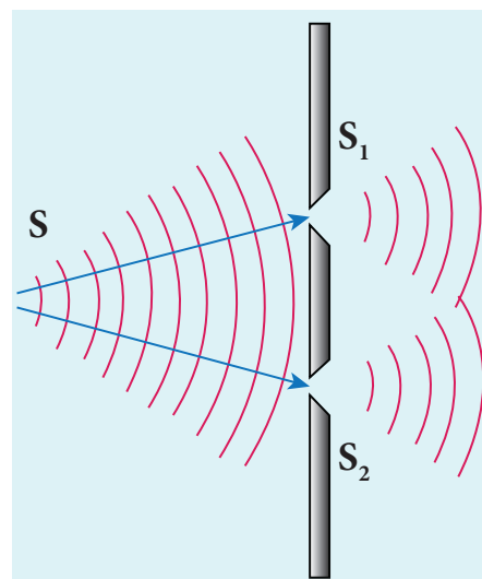
Figure 7.8 Wavefront division
