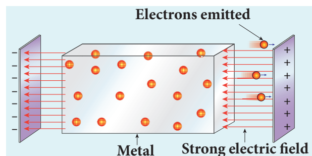
Figure 8.3 Field emission
