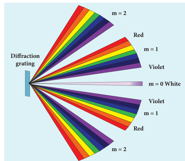
Figure 7.22 Diffraction with white light
