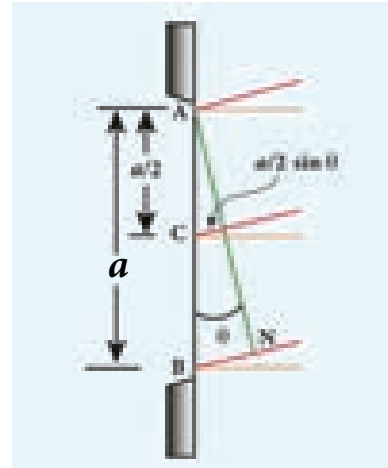
Figure 7.18 Corresponding points
