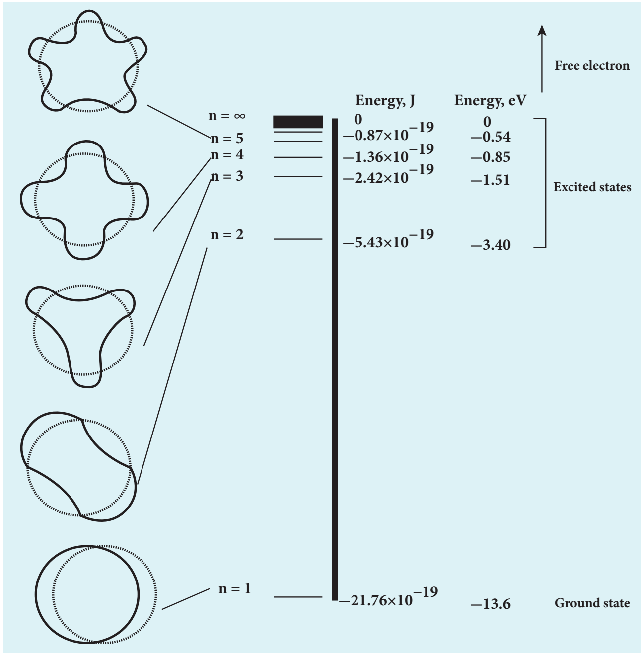
Figure 9.20 Energy levels of a hydrogen atom
