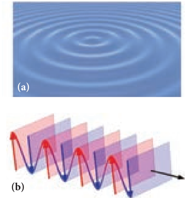
Figure 7.1 (a) Ripples on water surface (b) Wavefront and ray
