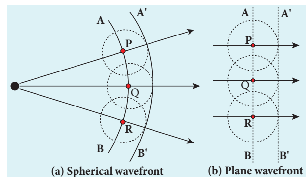
Figure 7.3 Huygens' Principle
