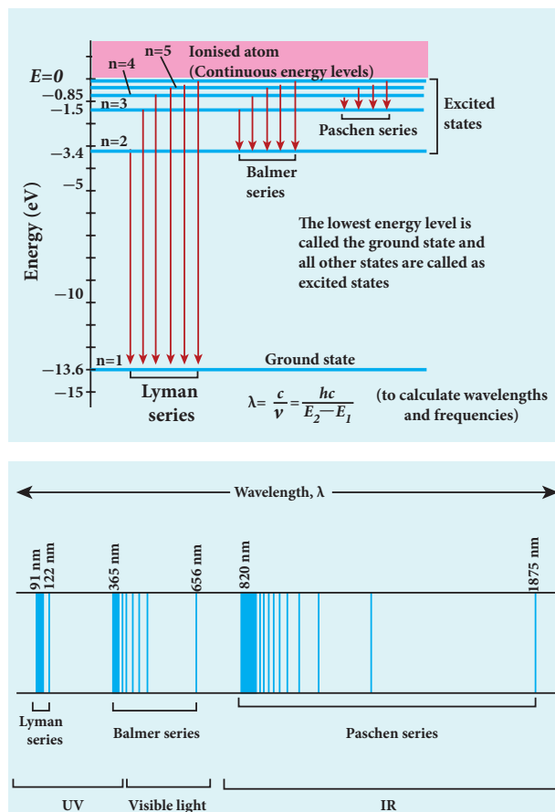
Figure 9.23 Spectral series – Lyman, Balmer, Paschen series
