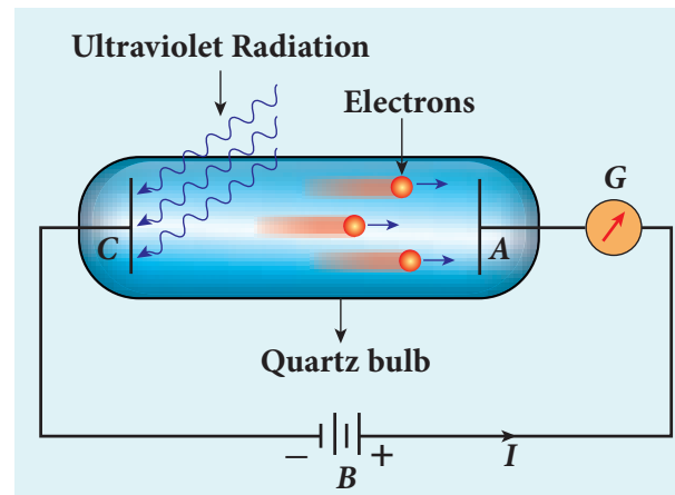
Figure 8.7 Experimental setup of Lenard
