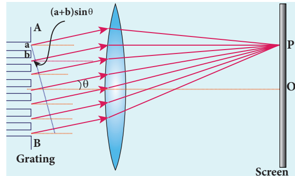
Figure 7.20 Diffraction grating experiment
