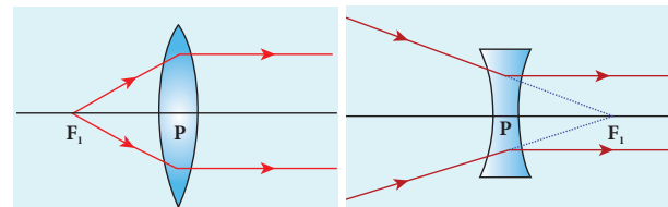
Figure 6.32 Primary focus
