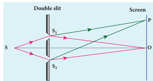
Figure 7.12 Young's double slit experimental setup
