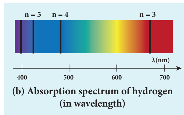
Figure 9.22 Hydrogen spectrum (a) emission (b) absorption
