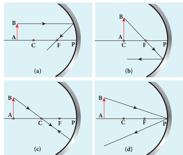
Figure 6.10 Image tracing
