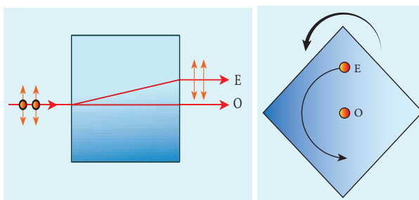
Figure 7.33 Double refraction
