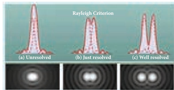
Figure 7.24 Rayleigh's criterion
