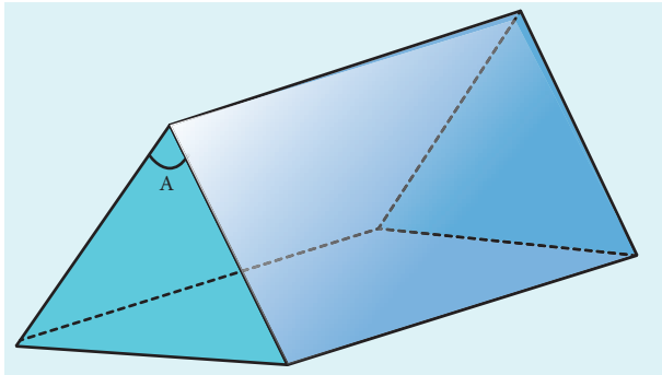
Figure 6.39 Prism
