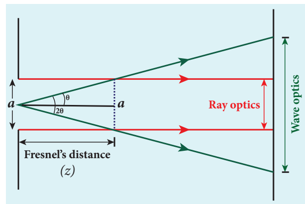
Figure 7.19 Fresnel's distance
