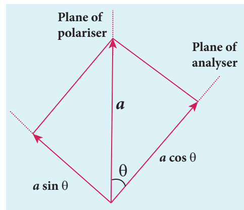
Figure 7.30 Malus' law
