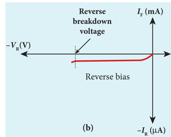
Figure 10.15 p - n junction diode
