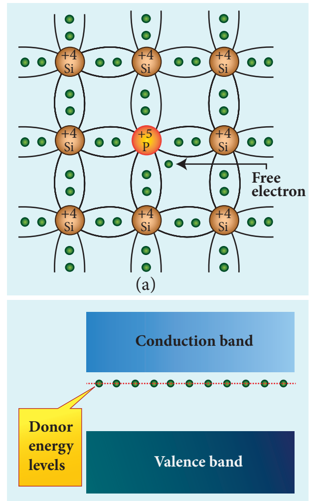
Figure 10.5 n -type extrinsic semiconductor: (a) Free electron which is loosely attached to the lattice (b) Representation of donor energy level
