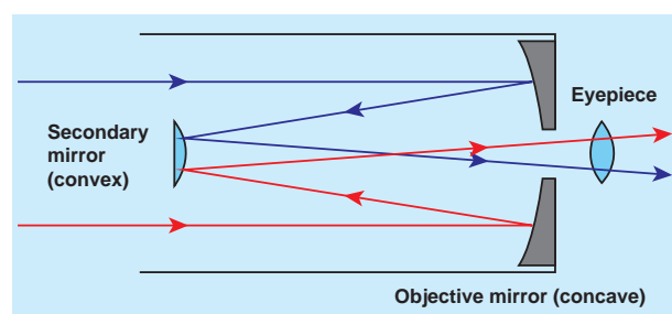
Figure 7.42 Reflecting telescope
