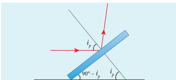
Figure 7.32 Pile of plates
