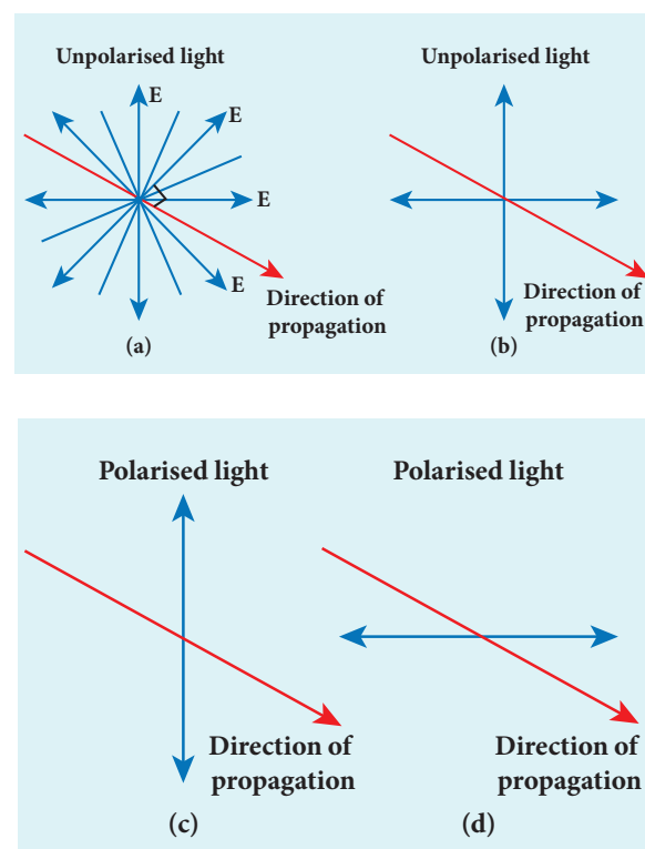
Figure 7.25 Unpolarised and polarised light
