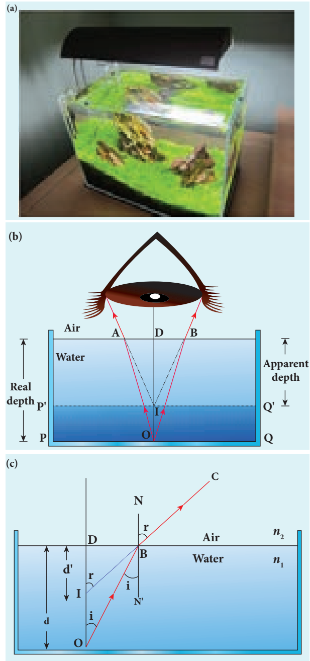
Figure 6.20 Apparent depth
